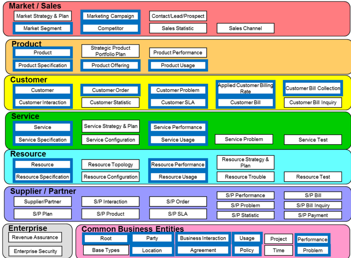
Figure 5-1 Information Framework: Level 1 ABEs in scope for OCDM V11.3.2 Assessment
